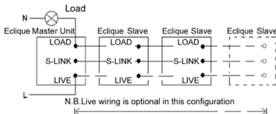
Fig 2. Wiring for Multi-Way Circuits
