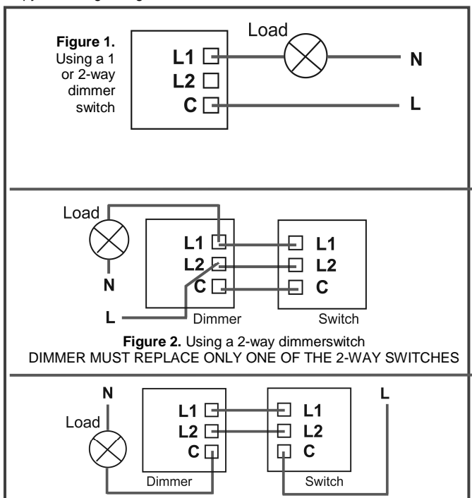
Figure 3. Using a 2-way dimmerswitch DIMMER MUST REPLACE ONLY ONE OF THE 2-WAY SWITCHES
