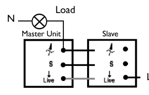
Fig 3. Alternative Wiring for Multi-Way Circuits
