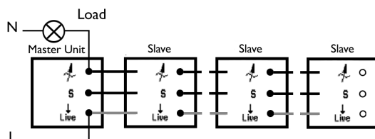
Fig 2. Wiring for Multi-Way Circuits
