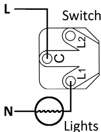
One way circuit
