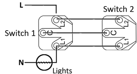
Two-way circuit (type 2)
