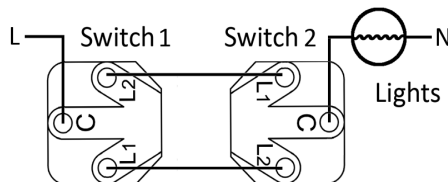
Two-way circuit (type 1)
